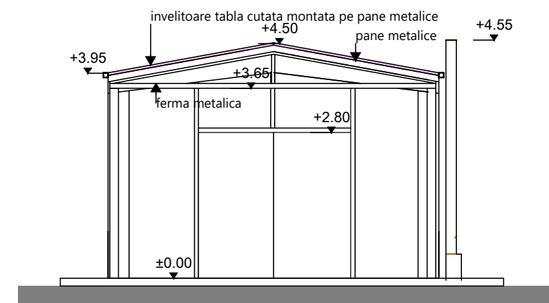
FATADA PRINCIPALA
